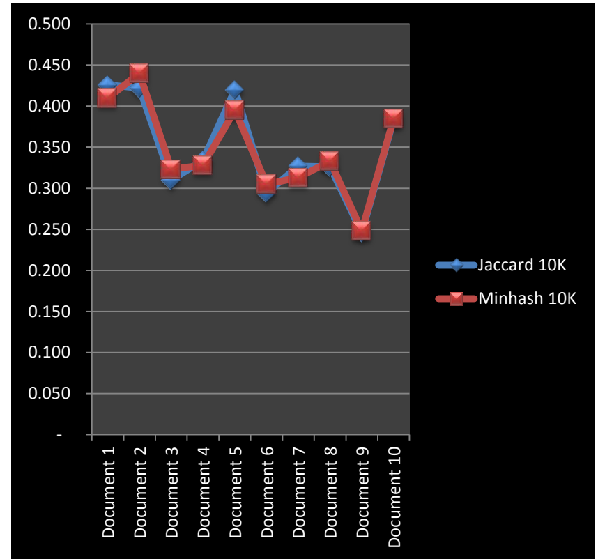
Jaccard Similarity
