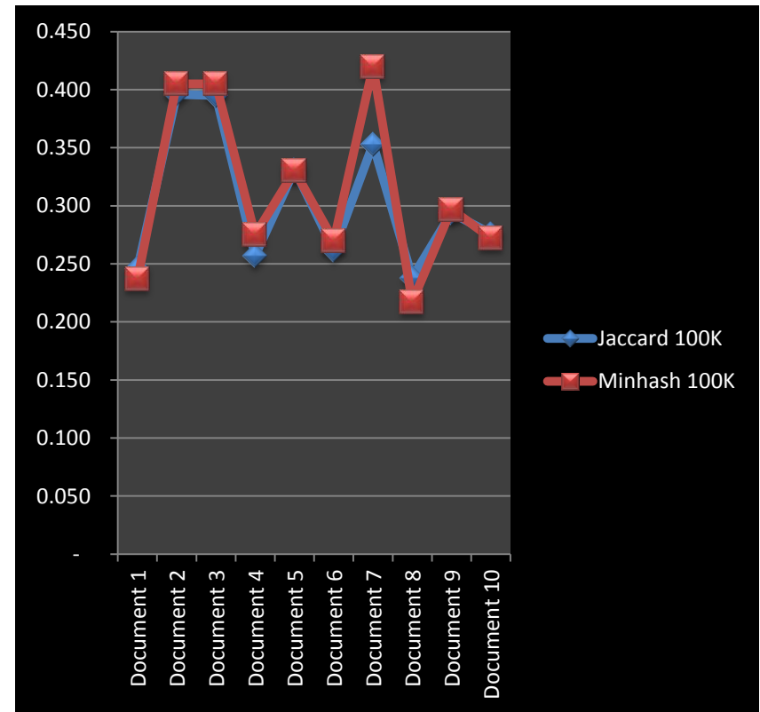
Jaccard Similarity
