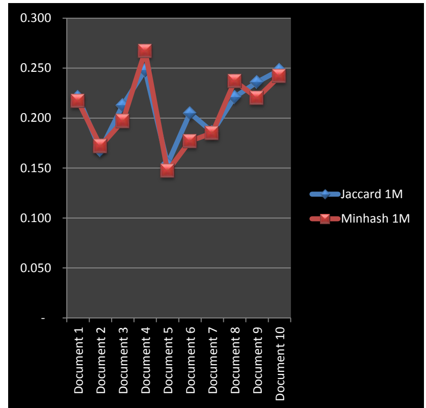
Jaccard Similarity
